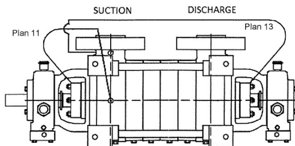
STANDARD PLAN 11/13
