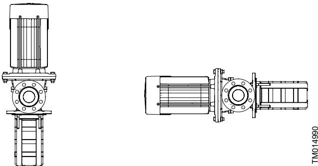
Installation of an MTR, MTRE pump
