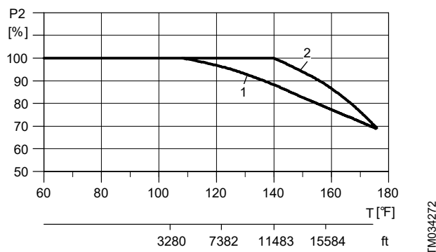
Relationship between motor output ( P_2 ) and ambient temperature/altitude
