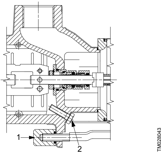
Horizontal installation
