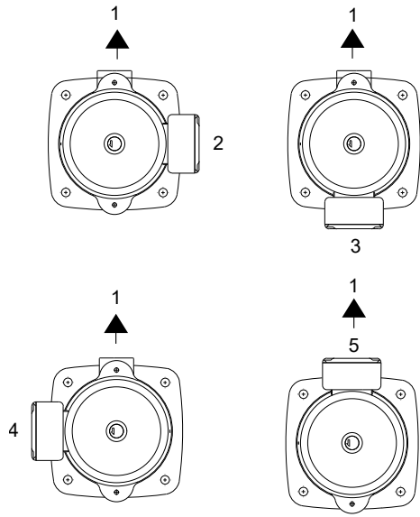
Possible terminal box positions
