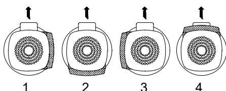
Terminal box positions, top view
