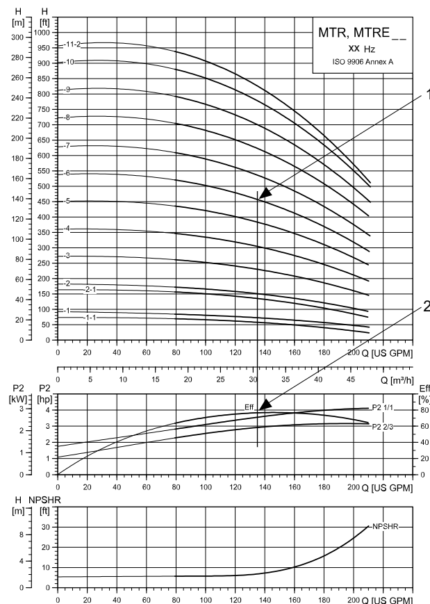
Example for the duty point of a pump
