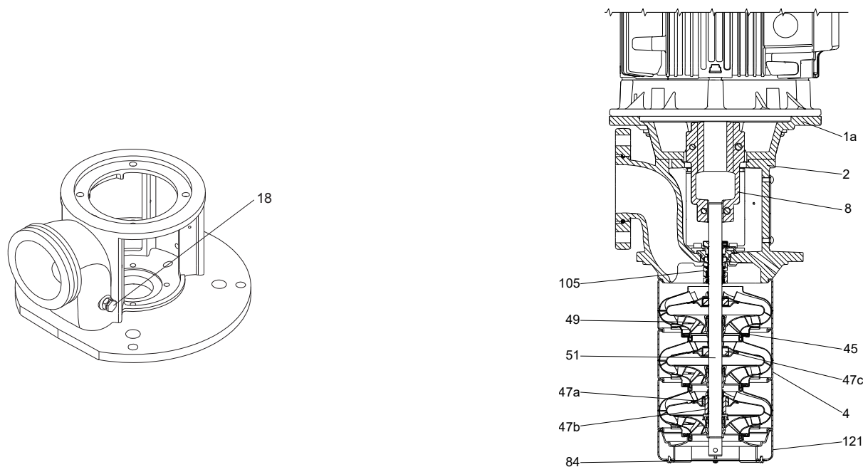
MTR, MTRE 32, 45 and 64
