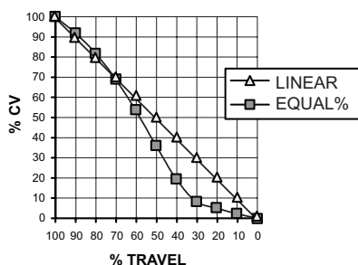
5840 & 5843 TYPICAL FLOW CURVES
