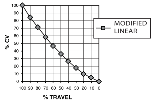
5848 FLOW CURVE
