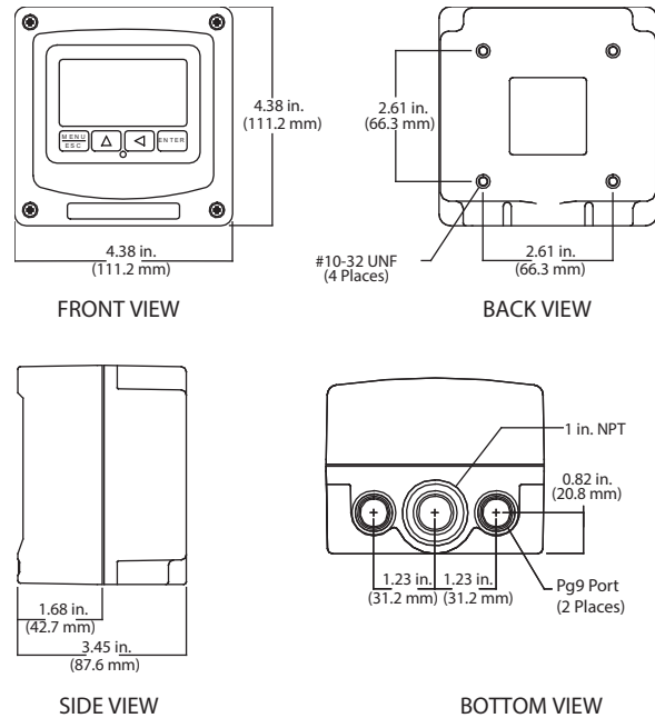
Figure 17: Q52/MetriNet enclosure dimensions
