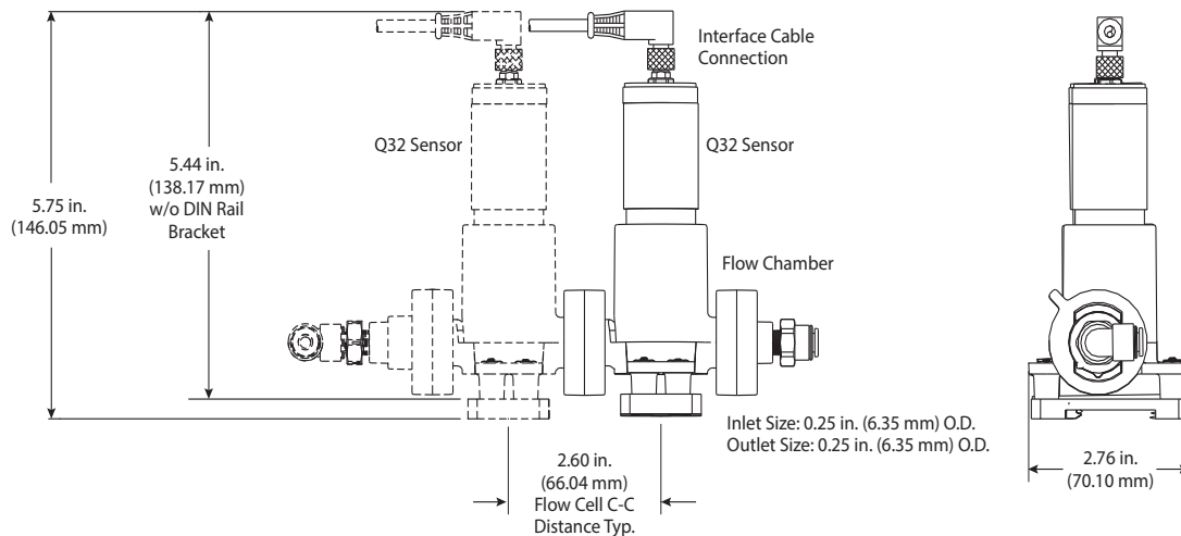
Figure 18: Q32 M-Node sensor flow cell dimensions
