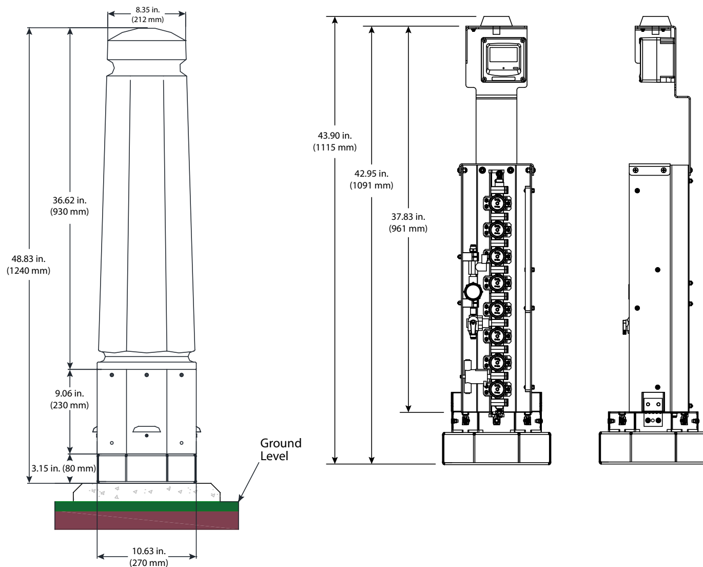
Figure 5: Bollard mount
