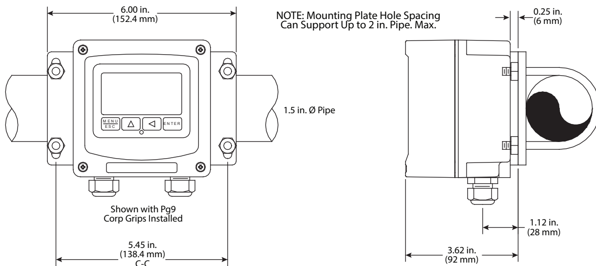
Figure 22: Pipe mount
