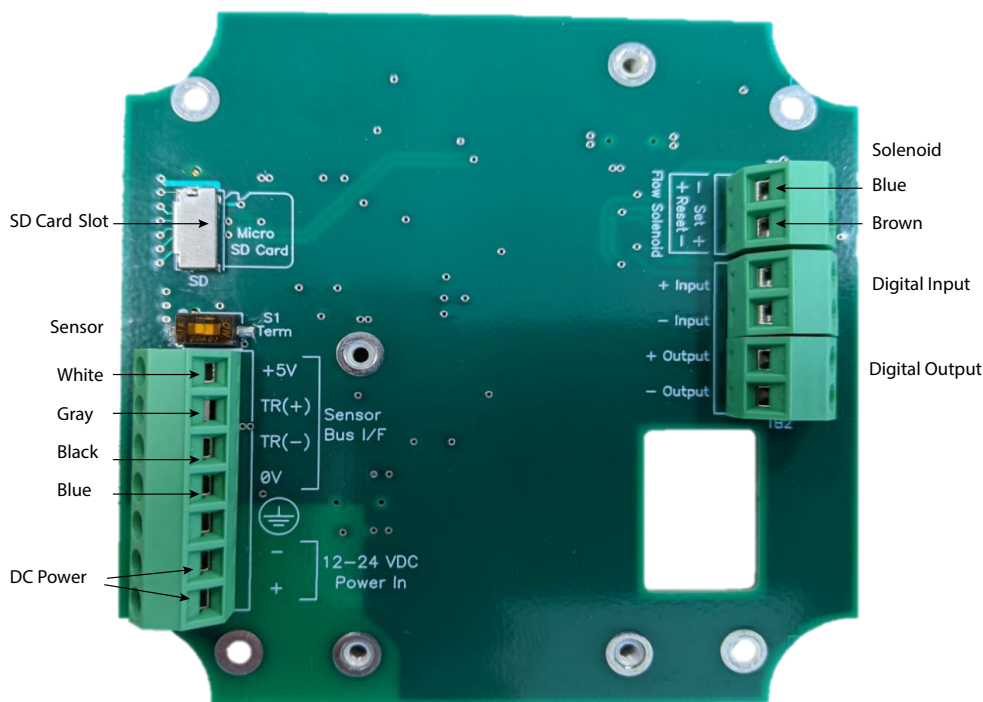
Figure 9: External connections
