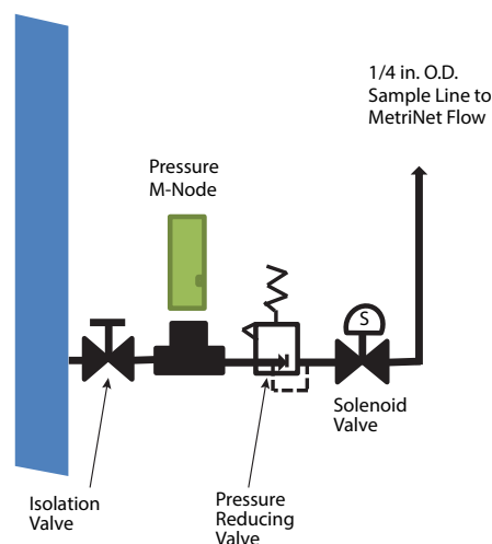
Figure 11: Possible user PRV/solenoid/shut-off assembly placement
