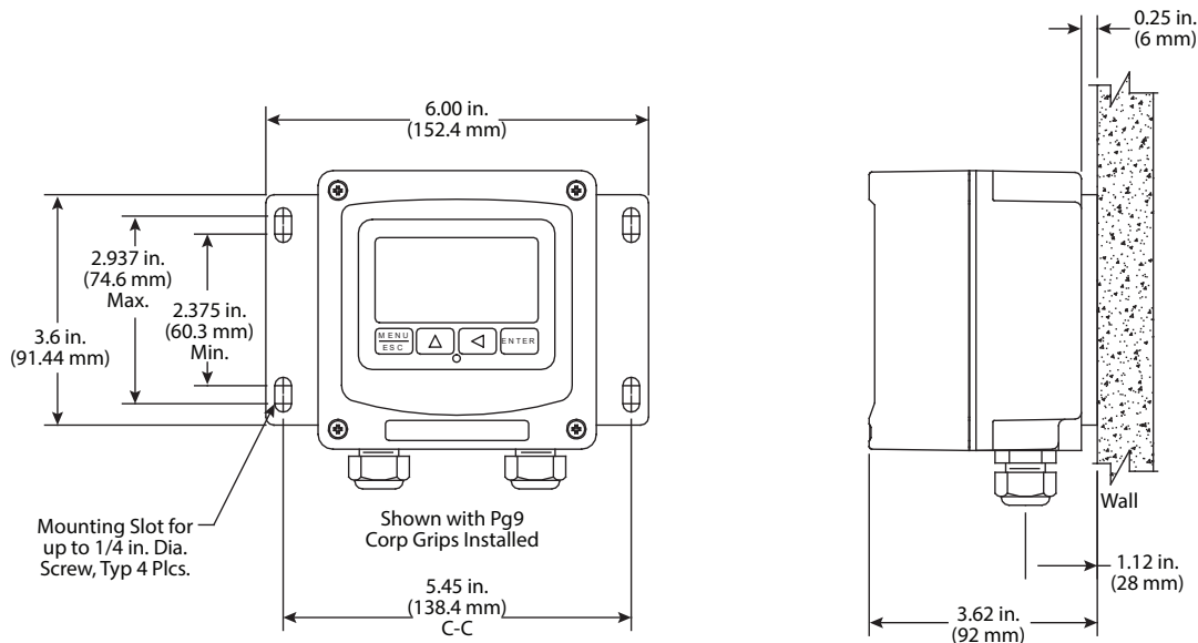
Figure 21: Wall mount
